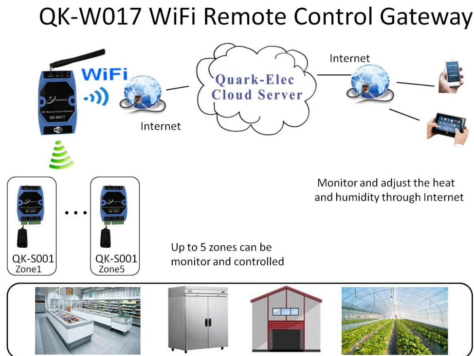
Figure 1 System diagram (Station mode)
